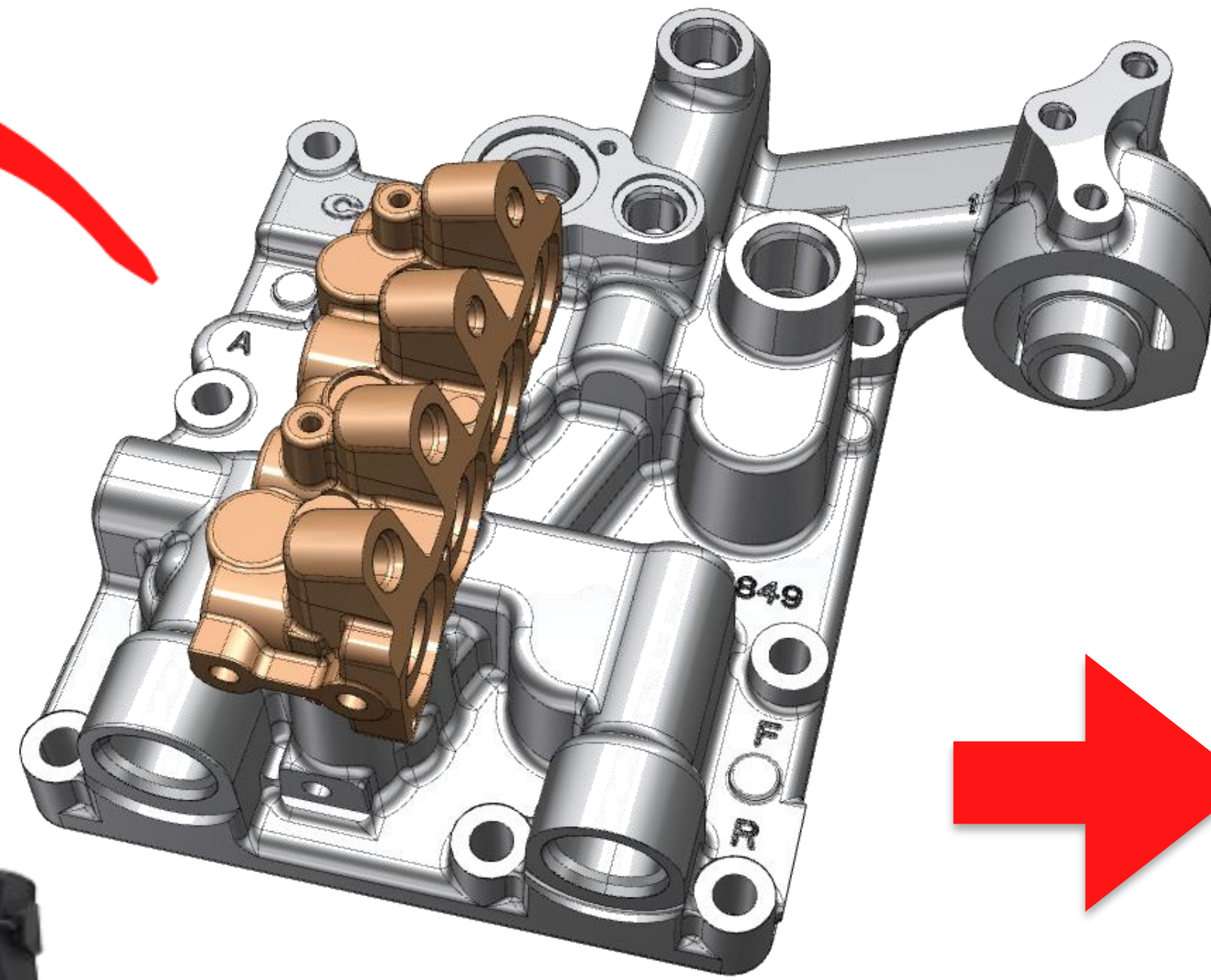
Conventional manifold
